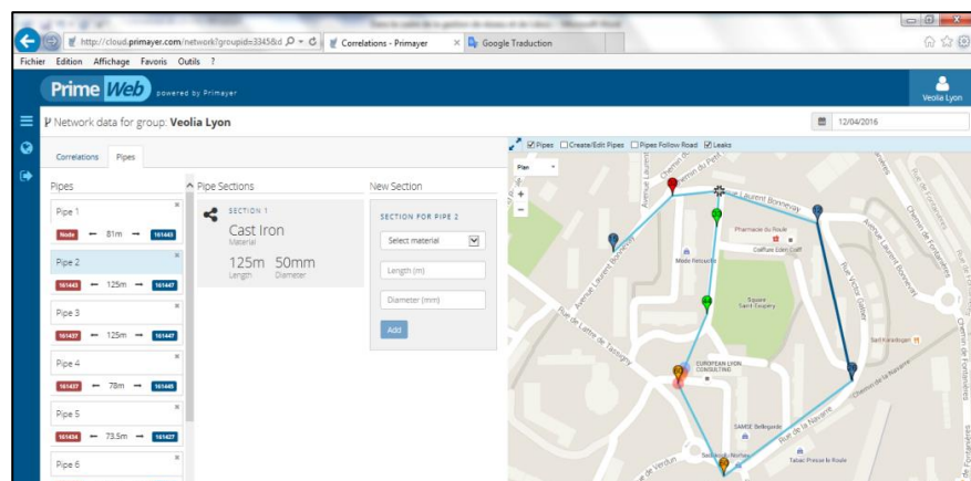
Network information on PrimeWeb tools
