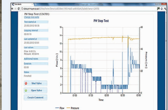
Graphing reduction detail in flow at each valve closure.
