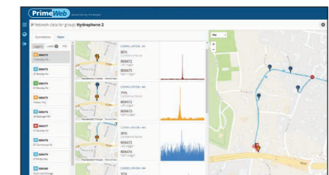
Multiple correlation results displayed with leak positions over distance of 614 metres.
