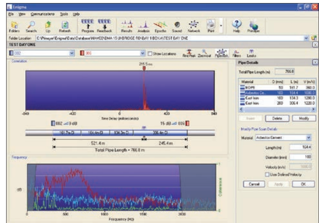
Leak on cast iron main found over 760m
