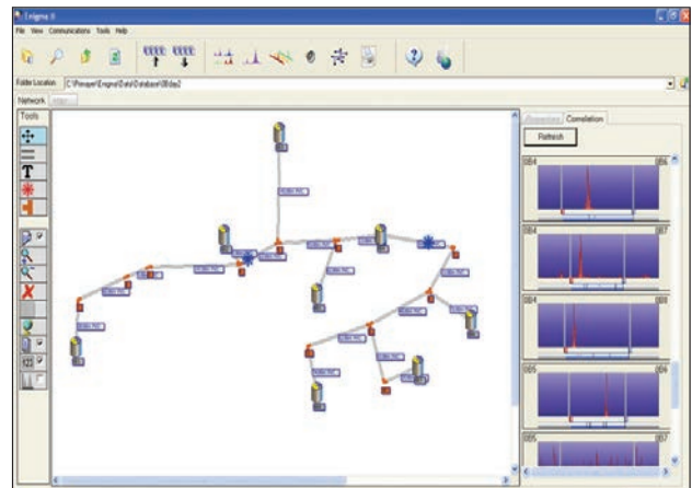
'Thumbnail' correlations displayed (right side of screen) with pipe schematic for easy visualisation of leaks and logger positions
